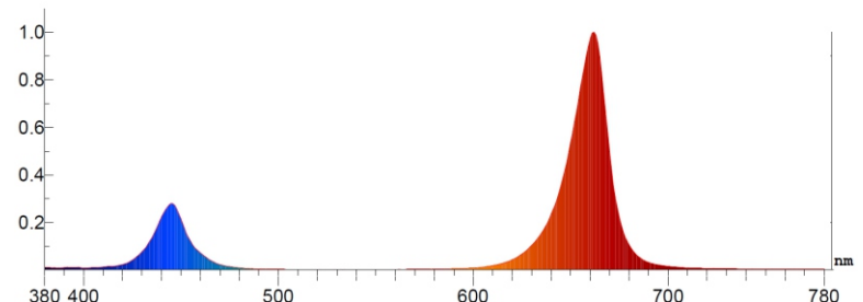
EXAMPLE: COLOR RATIO WITH DEFAULT 0.68:1 AT 100% ILLUMINANCE
