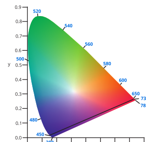
EXAMPLE: COLOR RATIO WITH DEFAULT 0.68:1 AT 100% ILLUMINANCE
