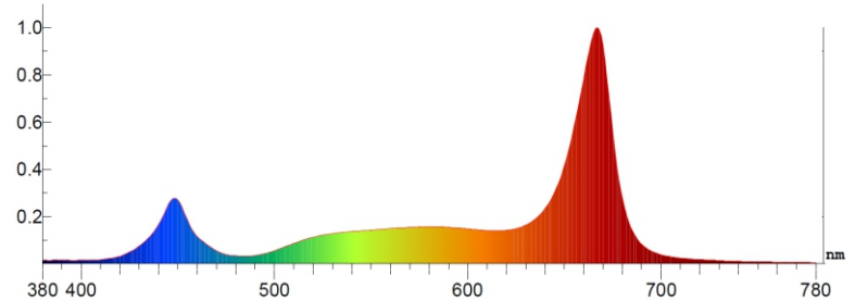
EXAMPLE COLOR RATIO WITH DEFAULT 6:1 AT 100% ILLUMINANCE
